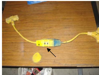
Figure 4: GFCI device for use with an extension cord for temporary service
